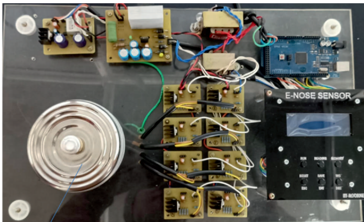
Development of basic electronic circuit for sensor
