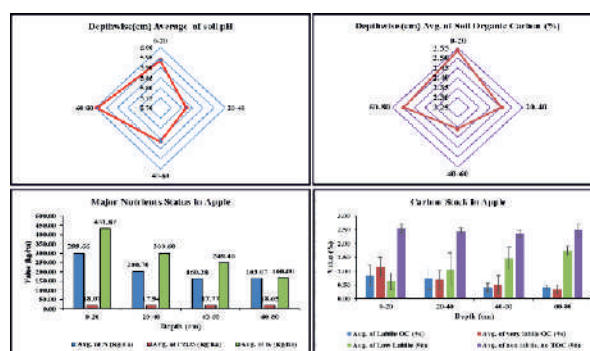
Fig 8. Soil pH, Organic Carbon, Major Nutrient Status and C stock in Apple orchards
